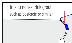
Typical Joint Detail
