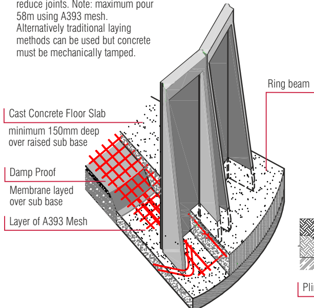
Typical part detail of plinth showing construction of floor slab
