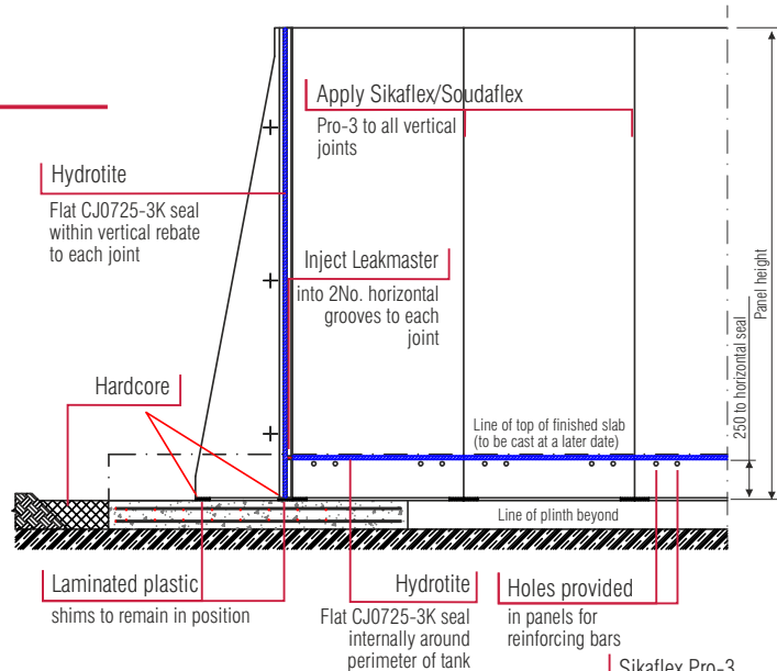
Typical Joint Detail
