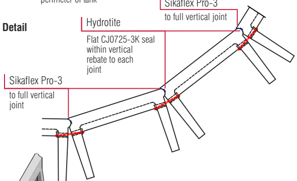
Typical part detail of plinth
